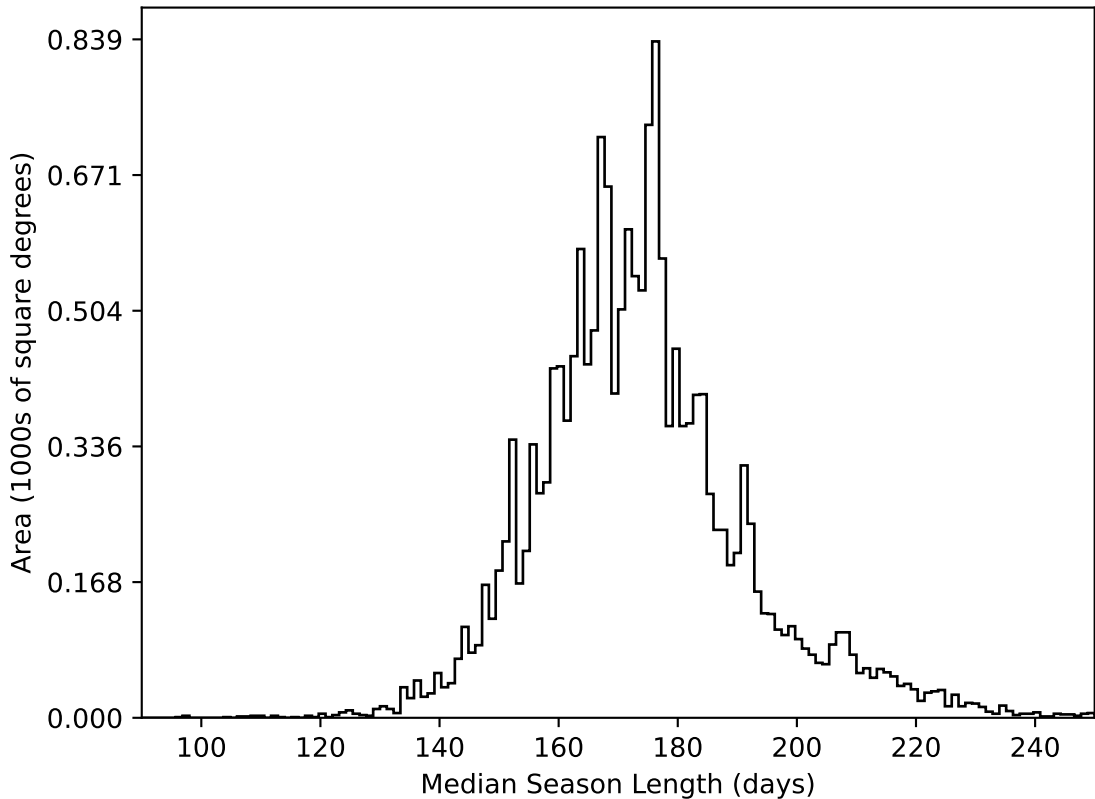
too_elab_r8_d2_ugrizy_v3.4_10yrs WFD all bands: Median Season Length
