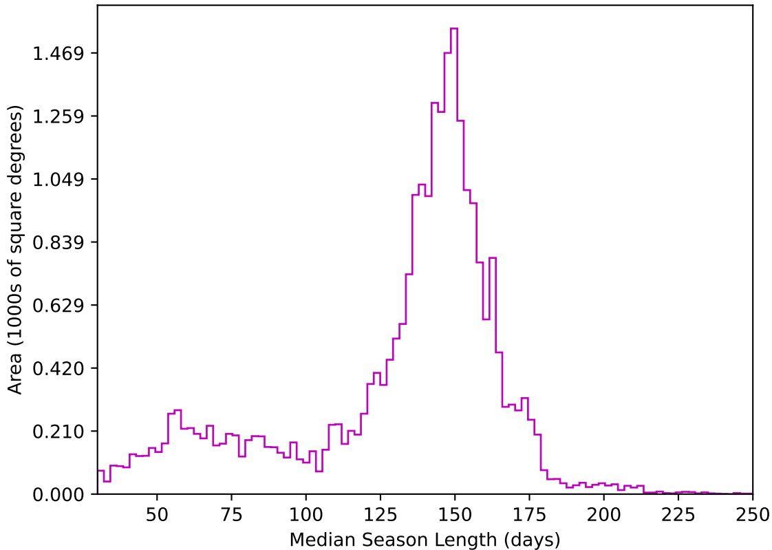
too_elab_r8_d2_ugrizy_v3.4_10yrs All sky z band: Median Season Length
