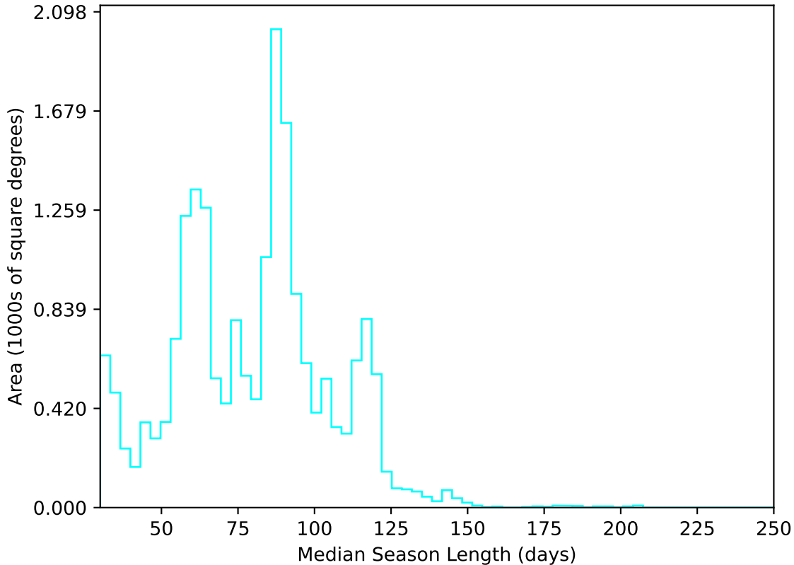
too_elab_r8_d2_ugrizy_v3.4_10yrs All sky u band: Median Season Length
