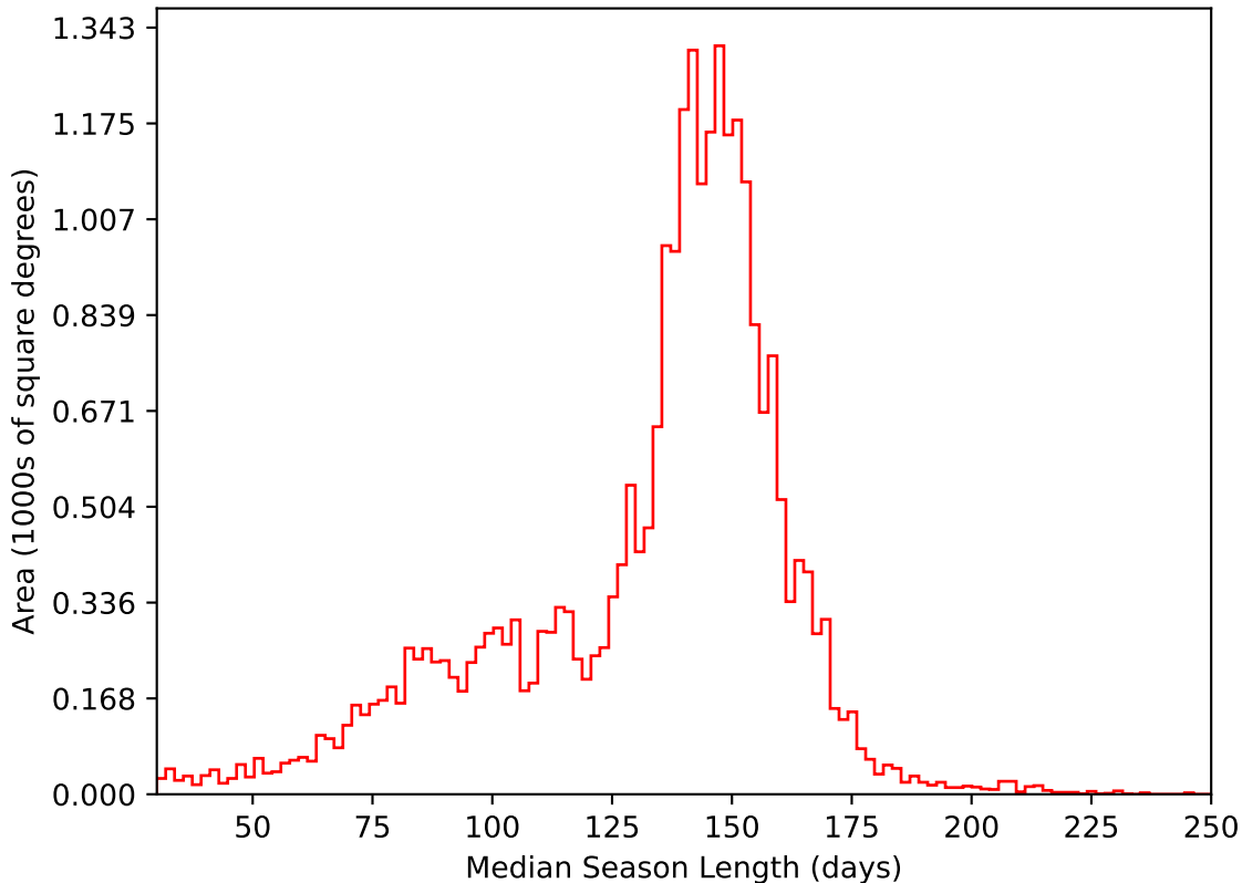
too_elab_r8_d2_ugrizy_v3.4_10yrs All sky i band: Median Season Length
