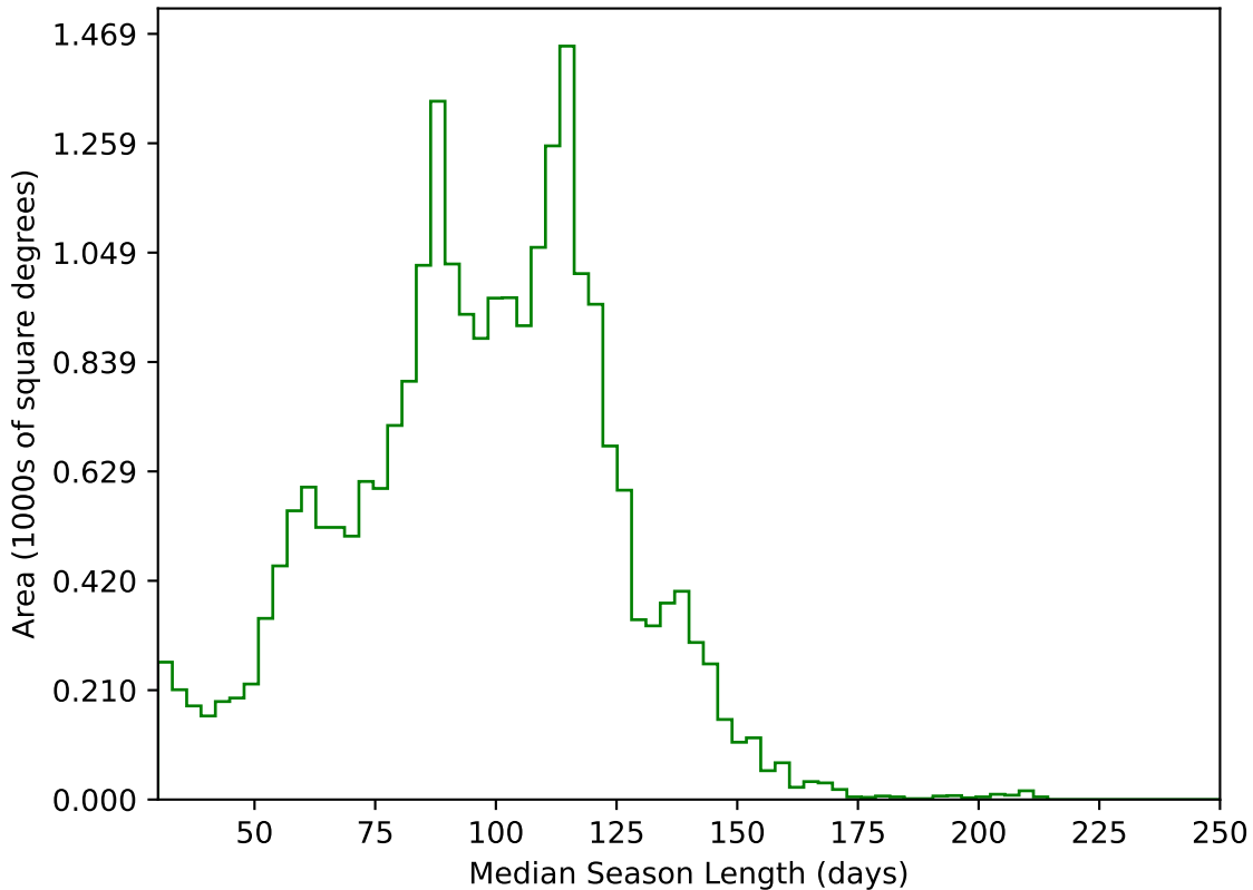
too_elab_r8_d2_ugrizy_v3.4_10yrs All sky g band: Median Season Length
