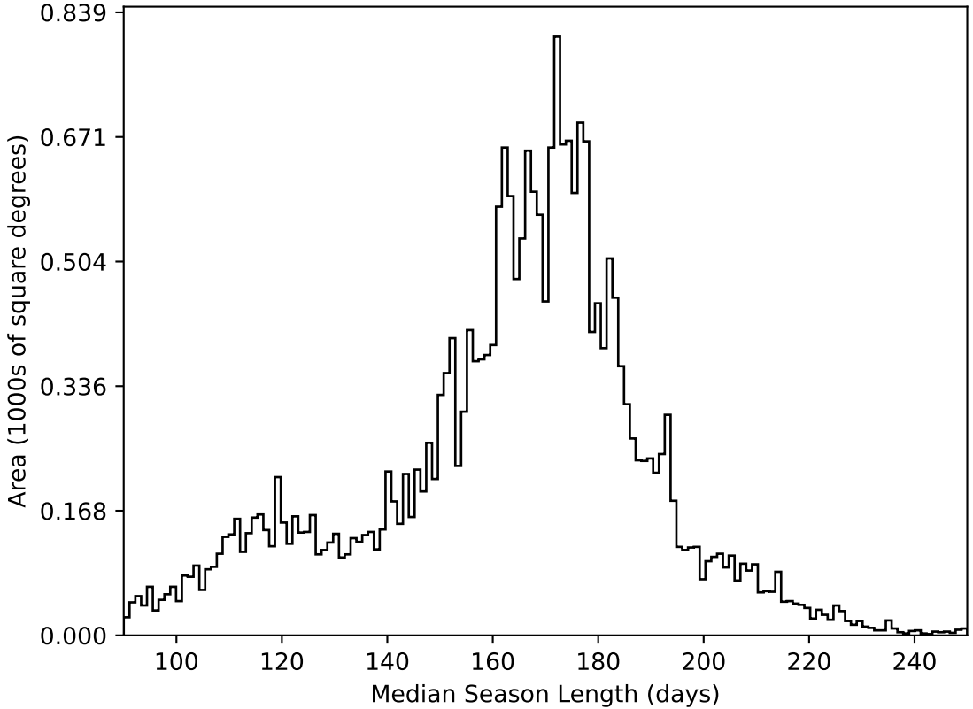
too_elab_r8_d2_ugrizy_v3.4_10yrs All sky all bands: Median Season Length
