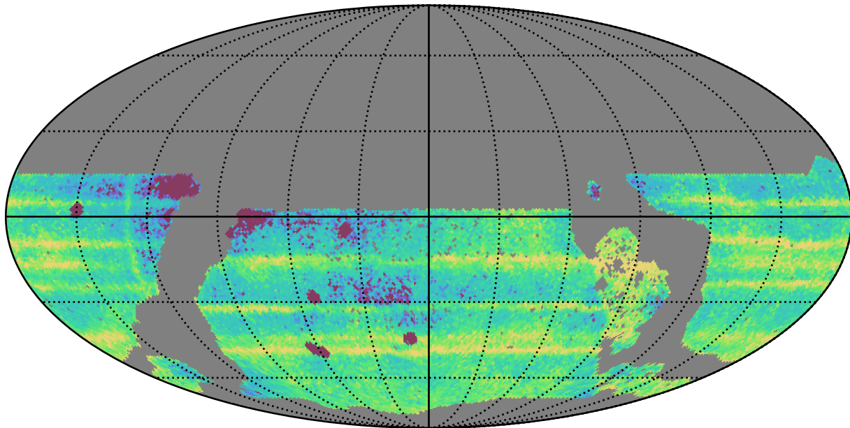
too_elab_r8_d2_ugrizy_v3.4_10yrs WFD: Median Intra-Night Gap
