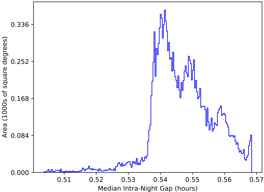
too_elab_r8_d2_ugrizy_v3.4_10yrs WFD: Median Intra-Night Gap
