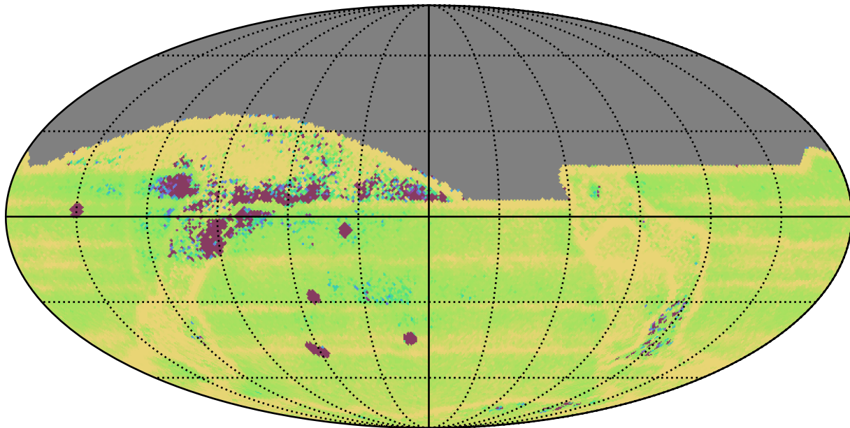
too_elab_r8_d2_ugrizy_v3.4_10yrs All sky: Median Intra-Night Gap
