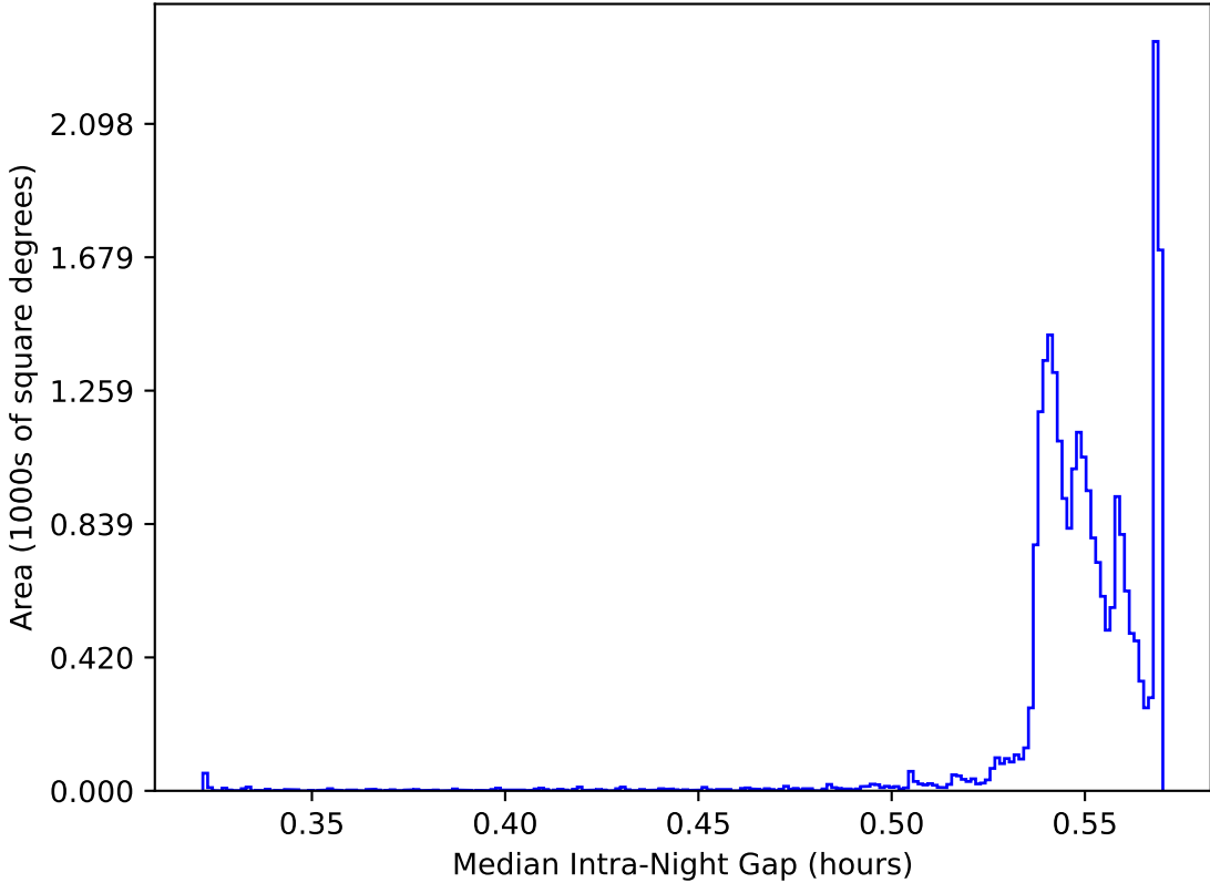
too_elab_r8_d2_ugrizy_v3.4_10yrs All sky: Median Intra-Night Gap
