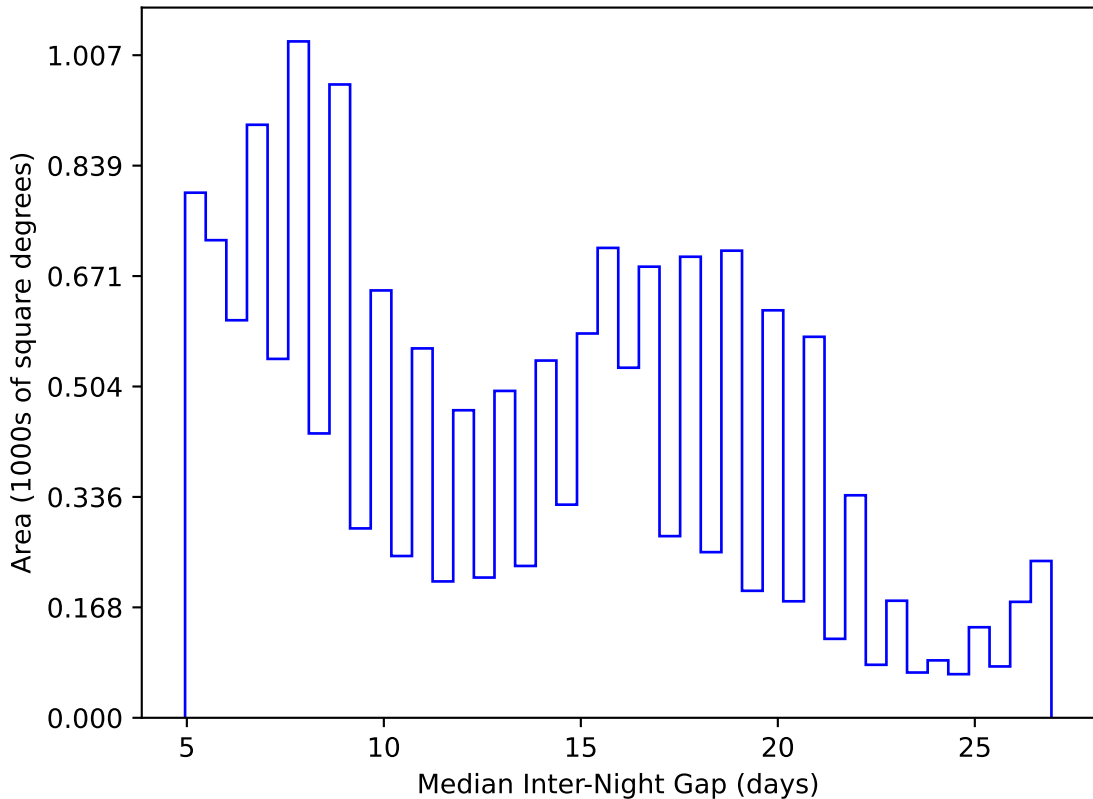
too_elab_r8_d2_ugrizy_v3.4_10yrs WFD y band: Median Inter-Night Gap
