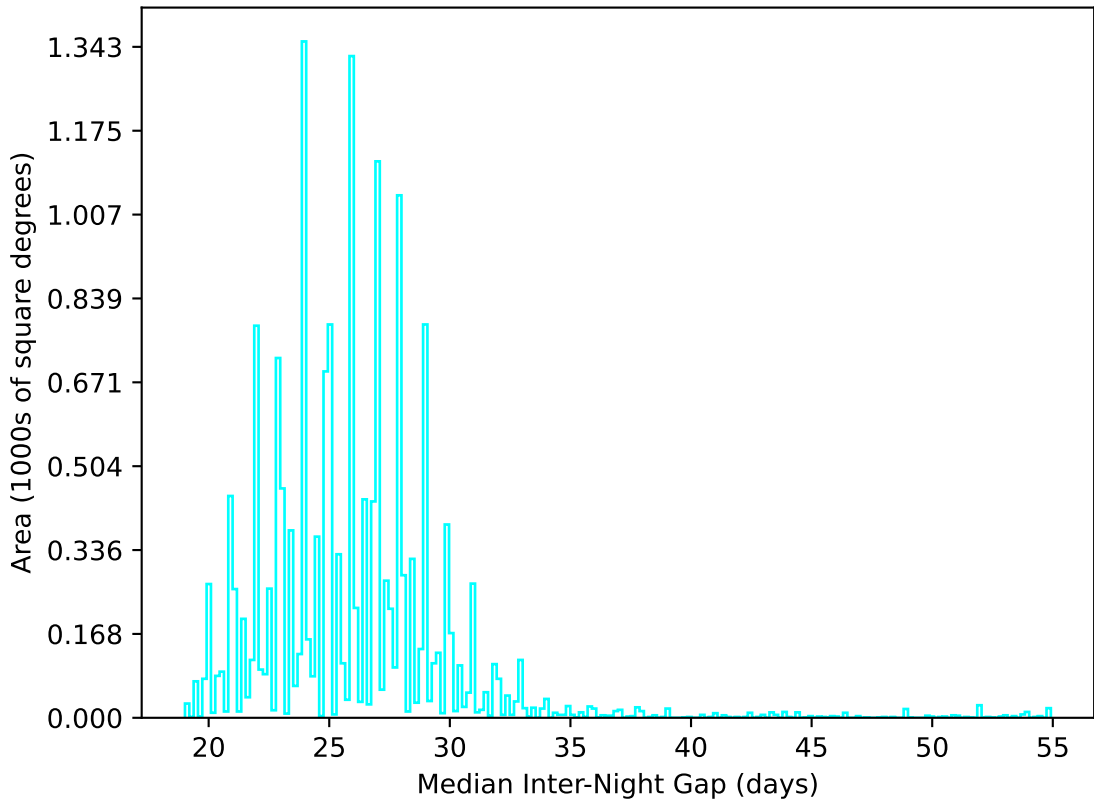
too_elab_r8_d2_ugrizy_v3.4_10yrs WFD u band: Median Inter-Night Gap
