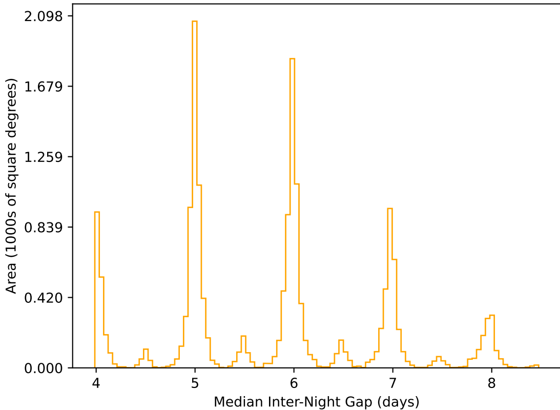
too_elab_r8_d2_ugrizy_v3.4_10yrs WFD r band: Median Inter-Night Gap
