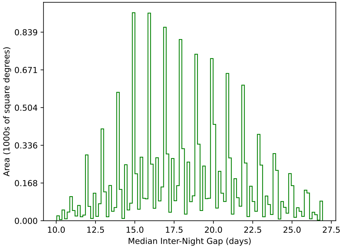
too_elab_r8_d2_ugrizy_v3.4_10yrs WFD g band: Median Inter-Night Gap
