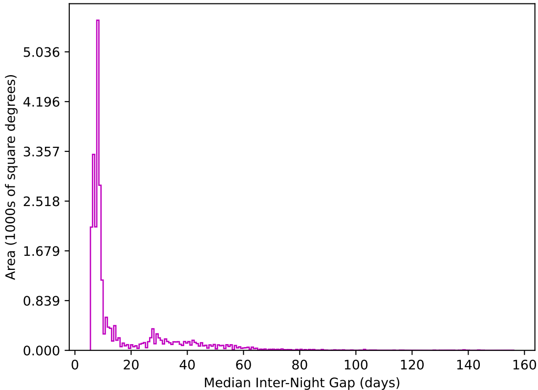
too_elab_r8_d2_ugrizy_v3.4_10yrs All sky z band: Median Inter-Night Gap
