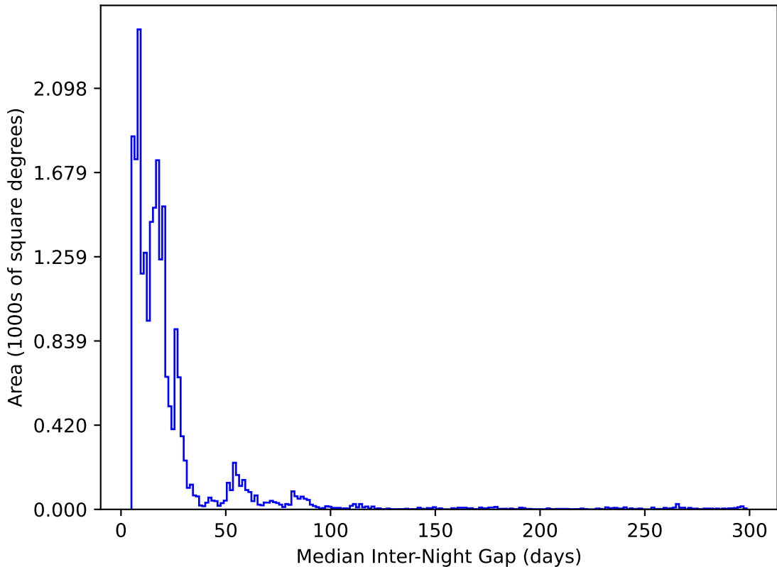
too_elab_r8_d2_ugrizy_v3.4_10yrs All sky y band: Median Inter-Night Gap
