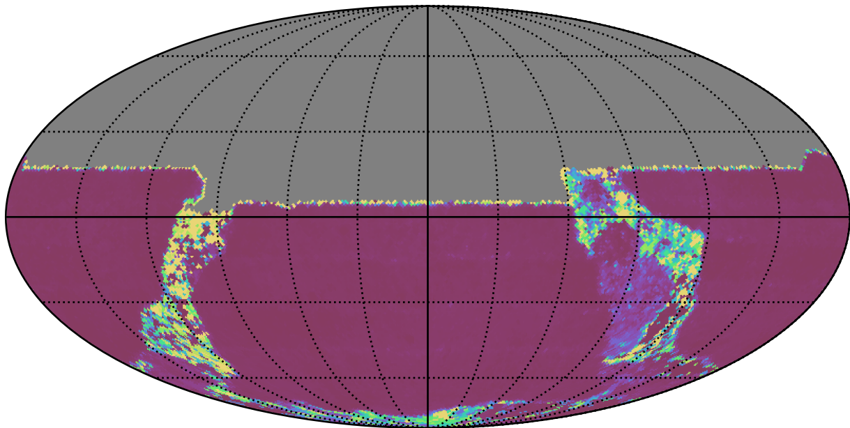
too_elab_r8_d2_ugrizy_v3.4_10yrs All sky u band: Median Inter-Night Gap
