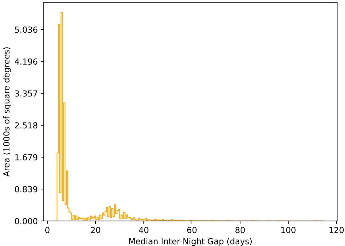
too_elab_r8_d2_ugrizy_v3.4_10yrs All sky r band: Median Inter-Night Gap
