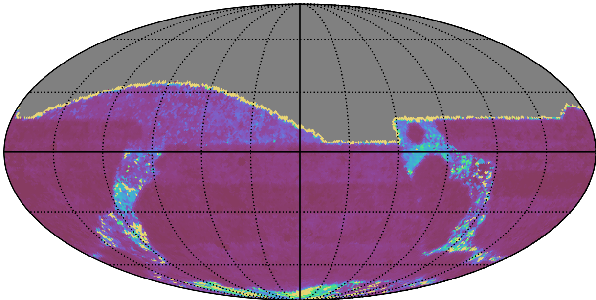
too_elab_r8_d2_ugrizy_v3.4_10yrs All sky g band: Median Inter-Night Gap
