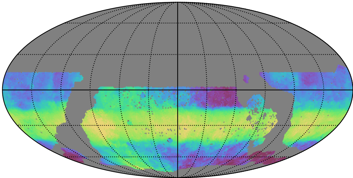
too_elab_r8_d2_ugrizy_v3.4_10yrs WFD z band: Median HA
