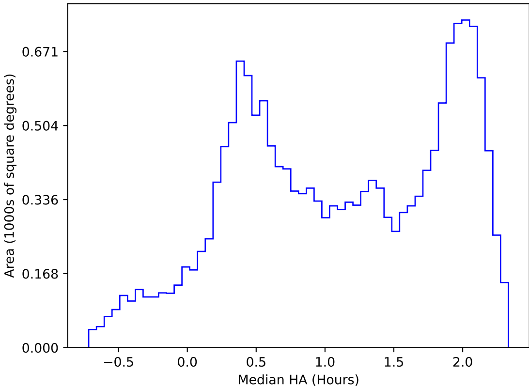
too_elab_r8_d2_ugrizy_v3.4_10yrs WFD z band: Median HA
