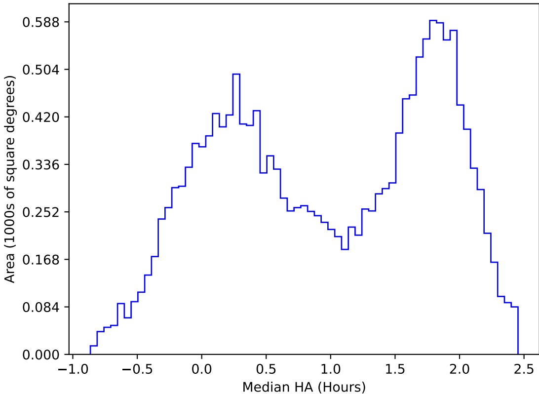
too_elab_r8_d2_ugrizy_v3.4_10yrs WFD u band: Median HA
