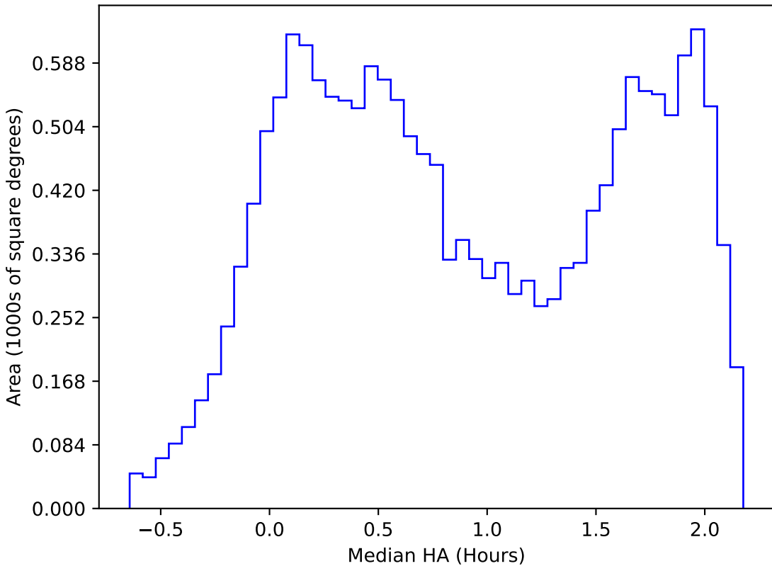
too_elab_r8_d2_ugrizy_v3.4_10yrs WFD r band: Median HA
