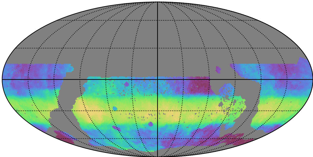
too_elab_r8_d2_ugrizy_v3.4_10yrs WFD i band: Median HA
