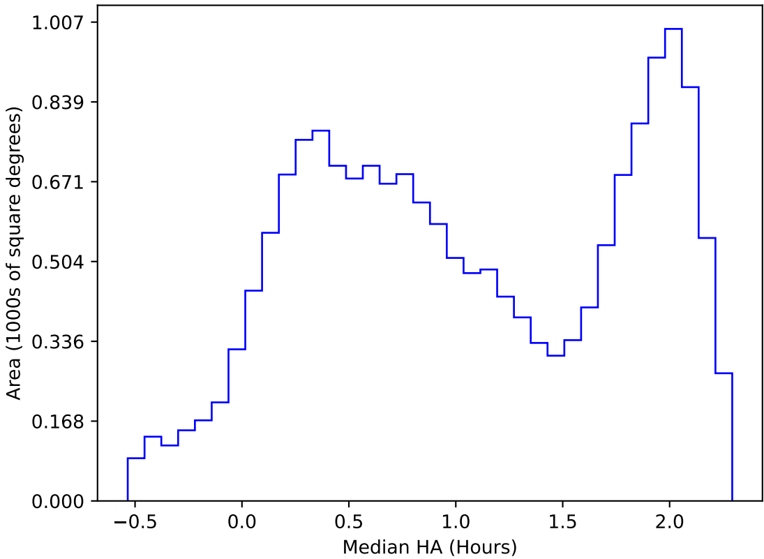
too_elab_r8_d2_ugrizy_v3.4_10yrs WFD i band: Median HA
