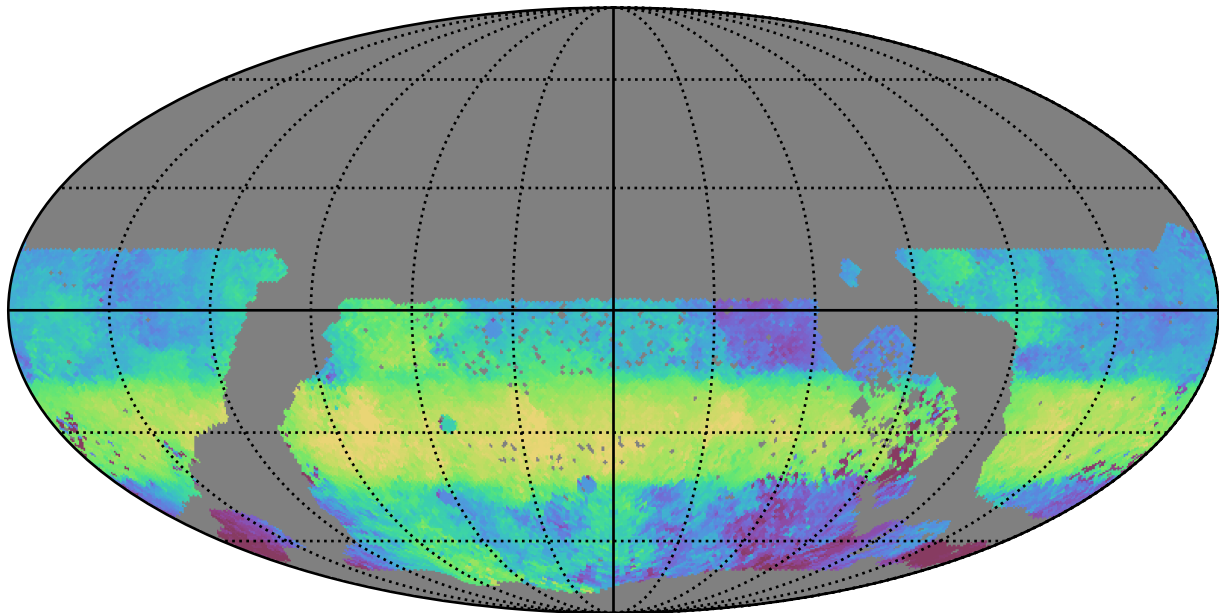
too_elab_r8_d2_ugrizy_v3.4_10yrs WFD g band: Median HA
