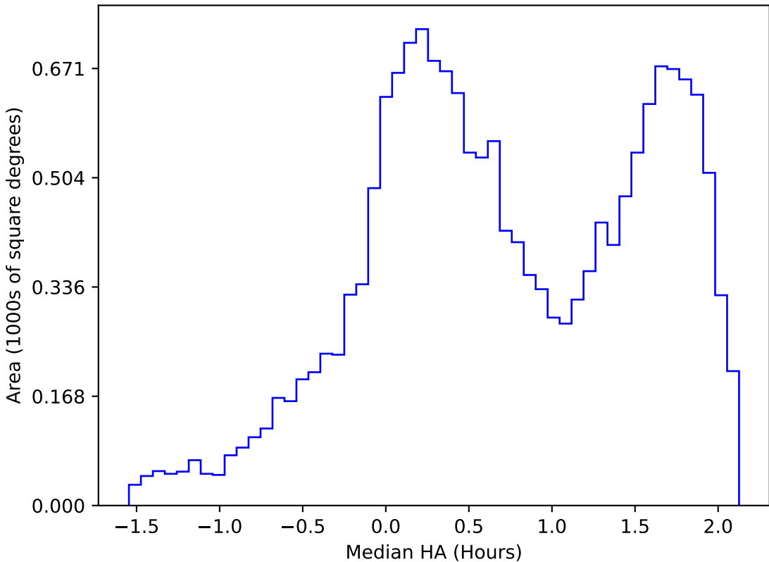
too_elab_r8_d2_ugrizy_v3.4_10yrs WFD g band: Median HA
