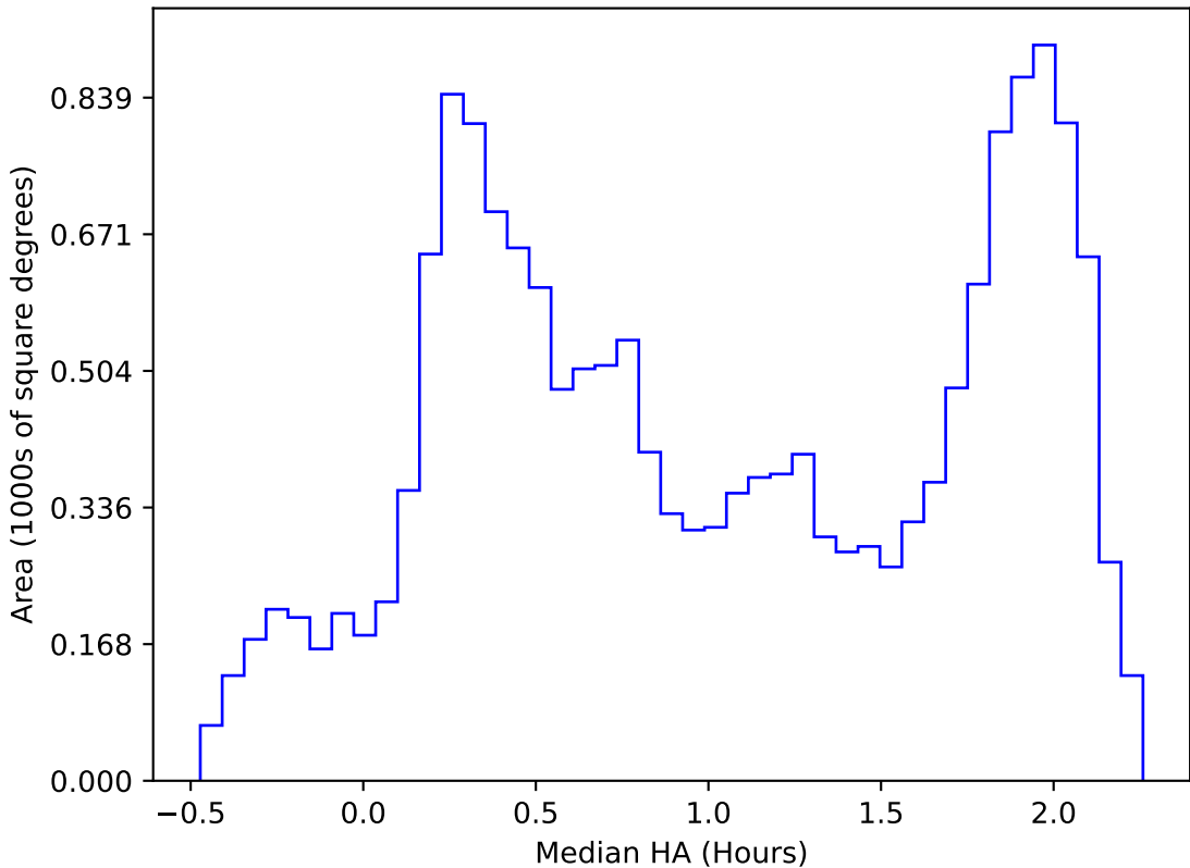
too_elab_r8_d2_ugrizy_v3.4_10yrs WFD all bands: Median HA
