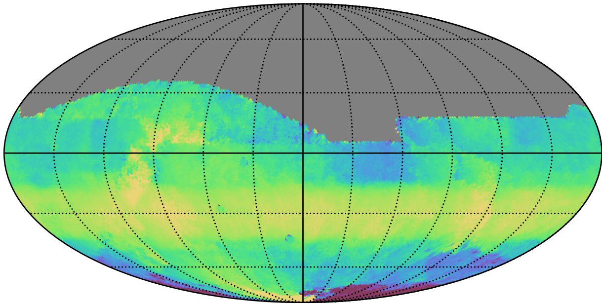
too_elab_r8_d2_ugrizy_v3.4_10yrs All sky z band: Median HA
