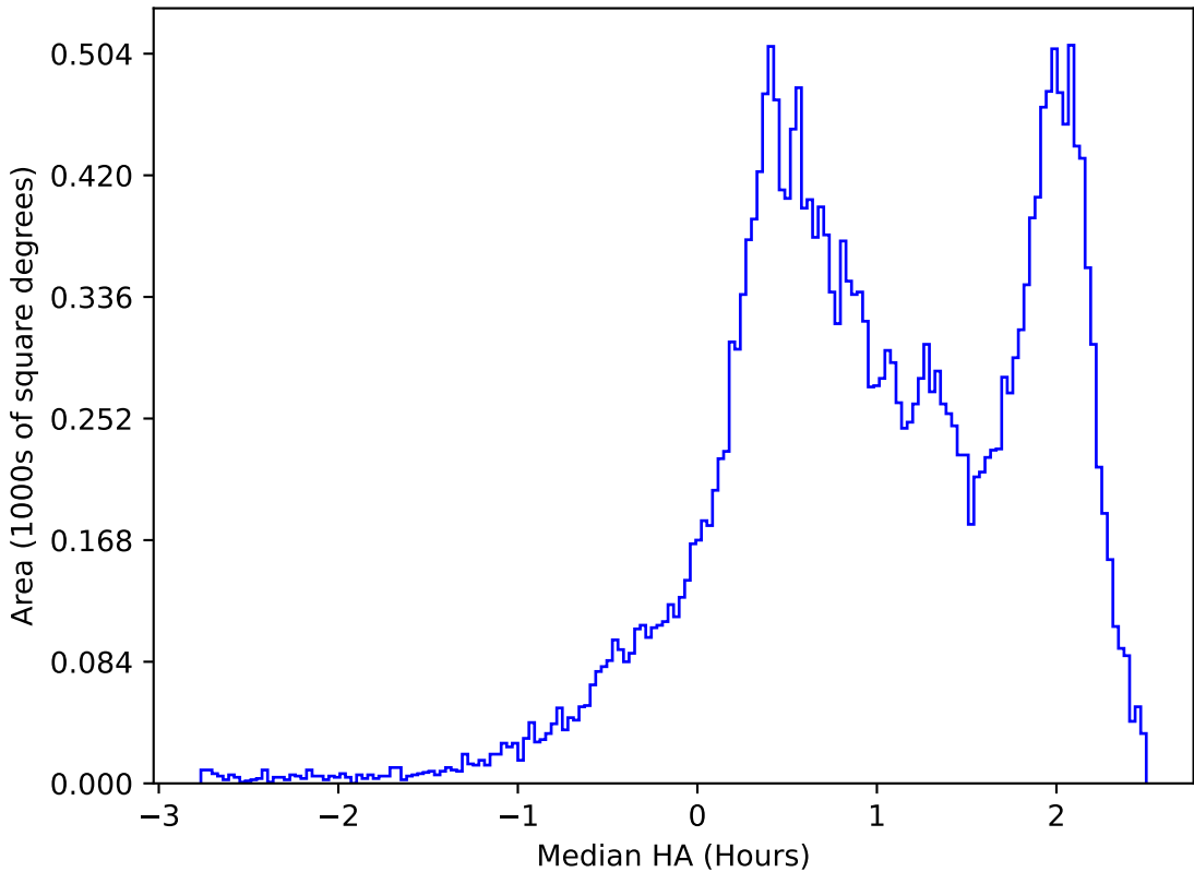
too_elab_r8_d2_ugrizy_v3.4_10yrs All sky z band: Median HA
