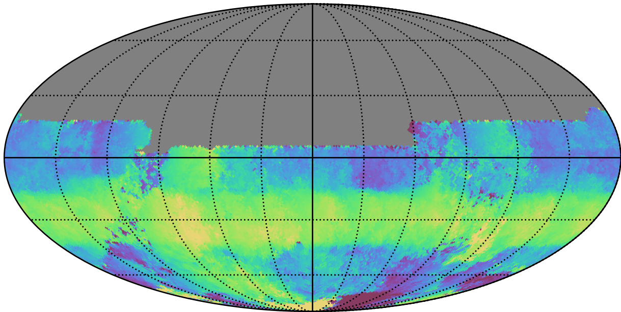
too_elab_r8_d2_ugrizy_v3.4_10yrs All sky u band: Median HA
