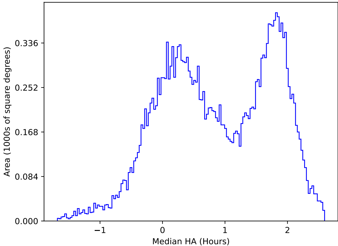
too_elab_r8_d2_ugrizy_v3.4_10yrs All sky u band: Median HA
