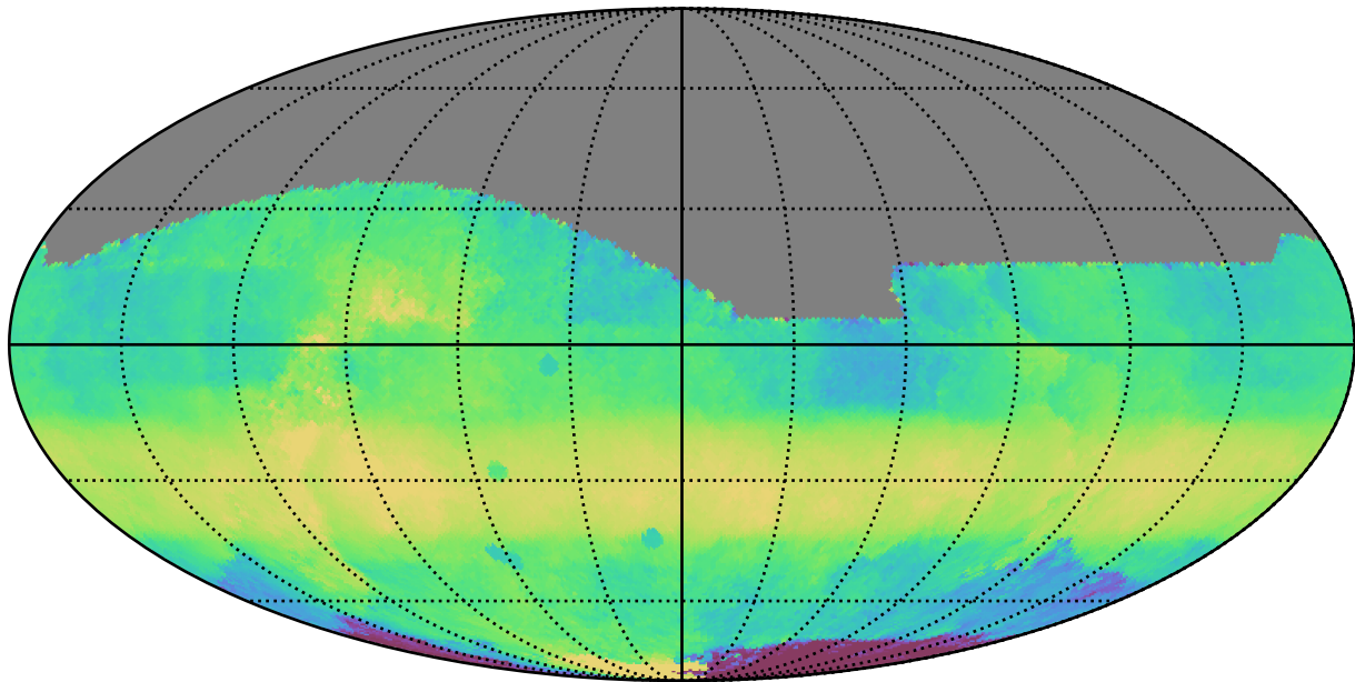
too_elab_r8_d2_ugrizy_v3.4_10yrs All sky i band: Median HA
