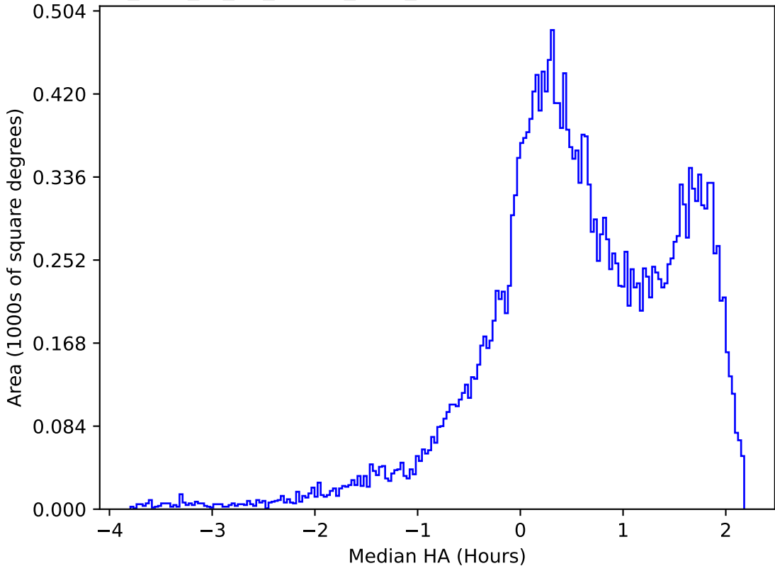
too_elab_r8_d2_ugrizy_v3.4_10yrs All sky g band: Median HA
