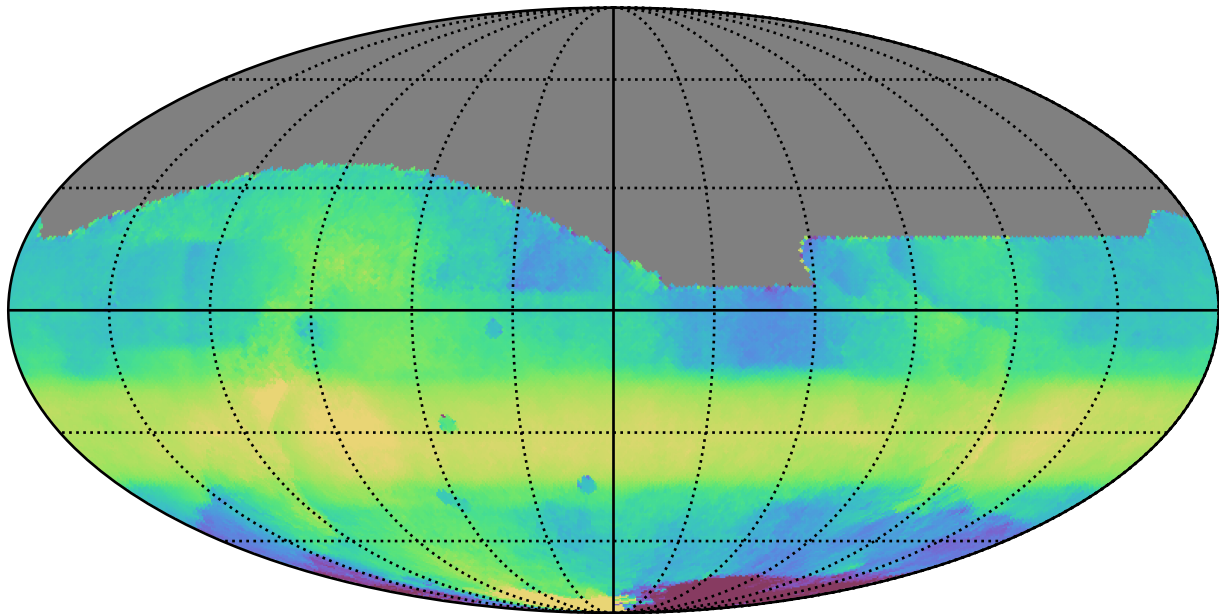
too_elab_r8_d2_ugrizy_v3.4_10yrs All sky all bands: Median HA
