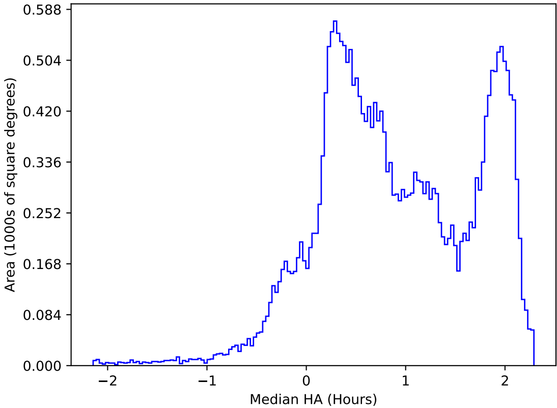
too_elab_r8_d2_ugrizy_v3.4_10yrs All sky all bands: Median HA
