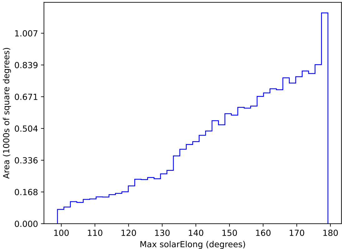
too_elab_r8_d2_ugrizy_v3.4_10yrs WFD z band: Max solarElong
