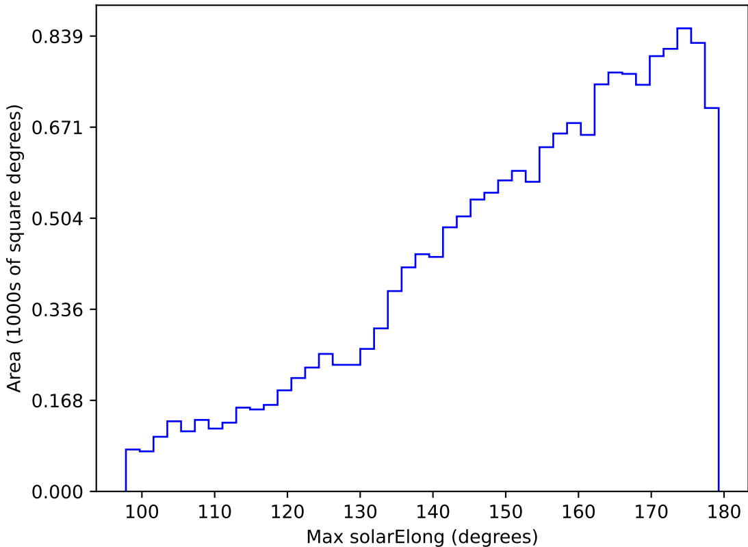
too_elab_r8_d2_ugrizy_v3.4_10yrs WFD u band: Max solarElong
