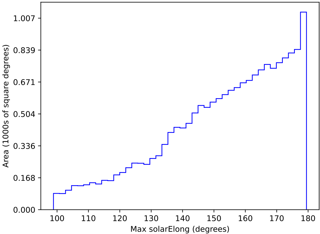
too_elab_r8_d2_ugrizy_v3.4_10yrs WFD r band: Max solarElong
