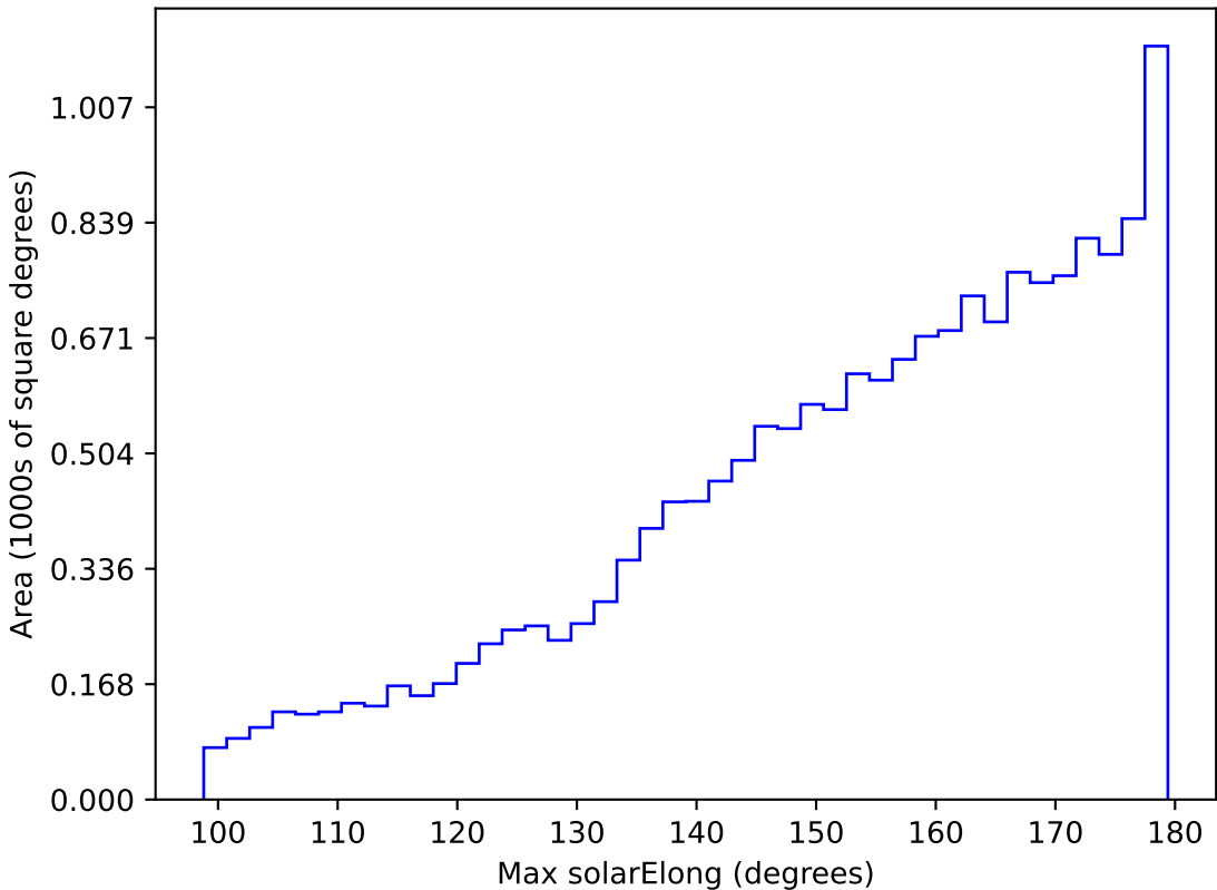
too_elab_r8_d2_ugrizy_v3.4_10yrs WFD i band: Max solarElong
