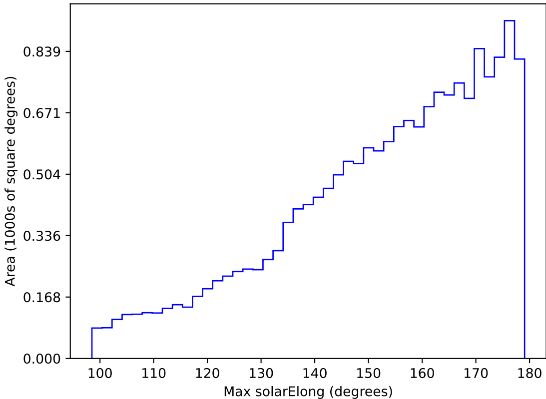
too_elab_r8_d2_ugrizy_v3.4_10yrs WFD g band: Max solarElong
