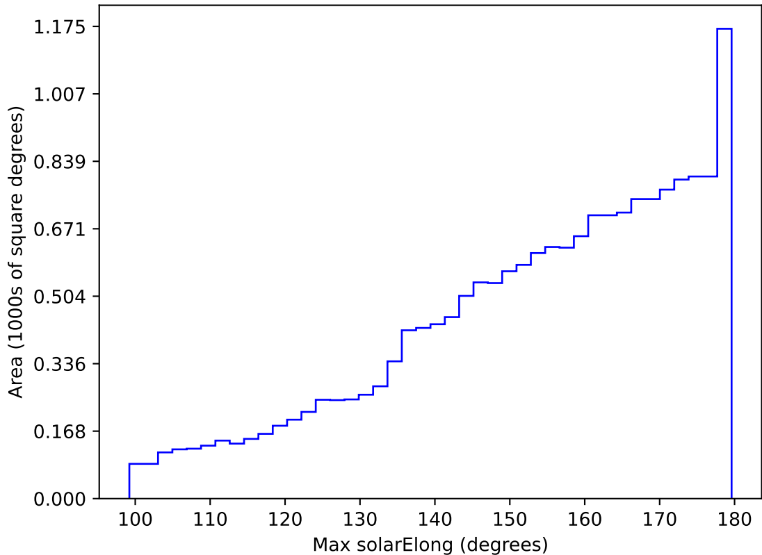
too_elab_r8_d2_ugrizy_v3.4_10yrs WFD all bands: Max solarElong
