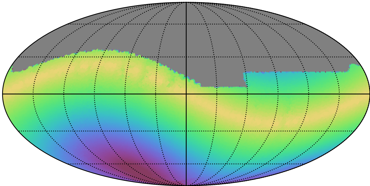
too_elab_r8_d2_ugrizy_v3.4_10yrs All sky z band: Max solarElong
