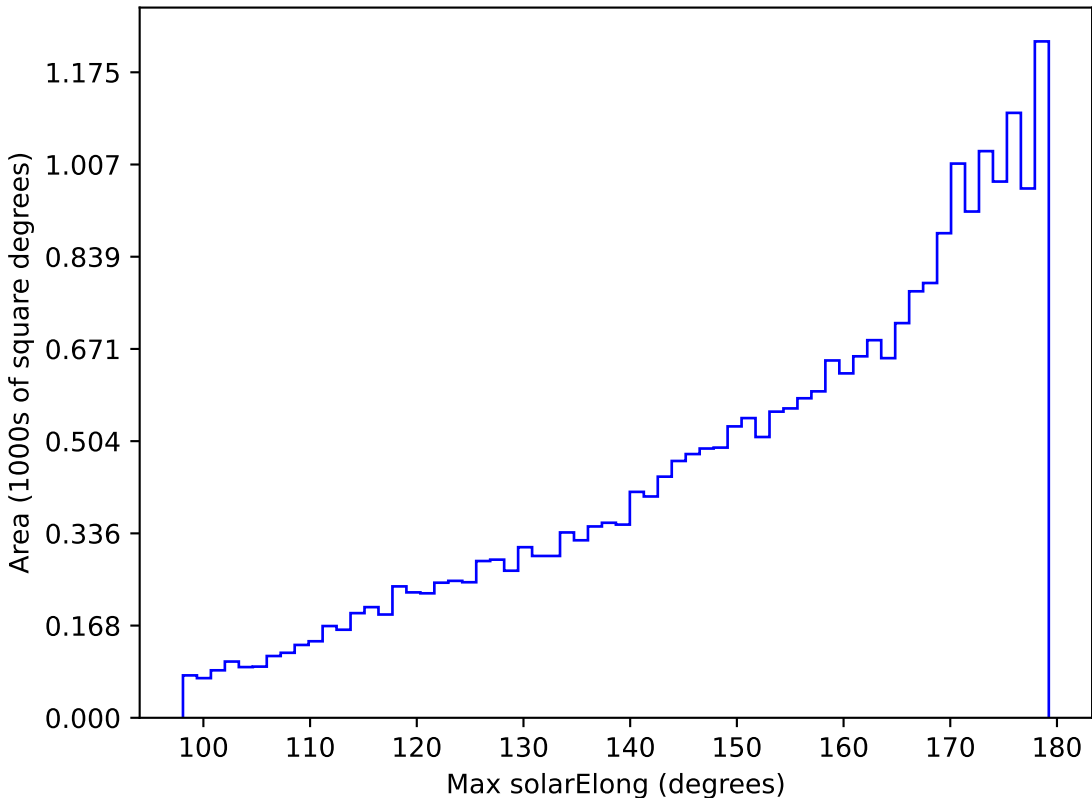
too_elab_r8_d2_ugrizy_v3.4_10yrs All sky z band: Max solarElong
