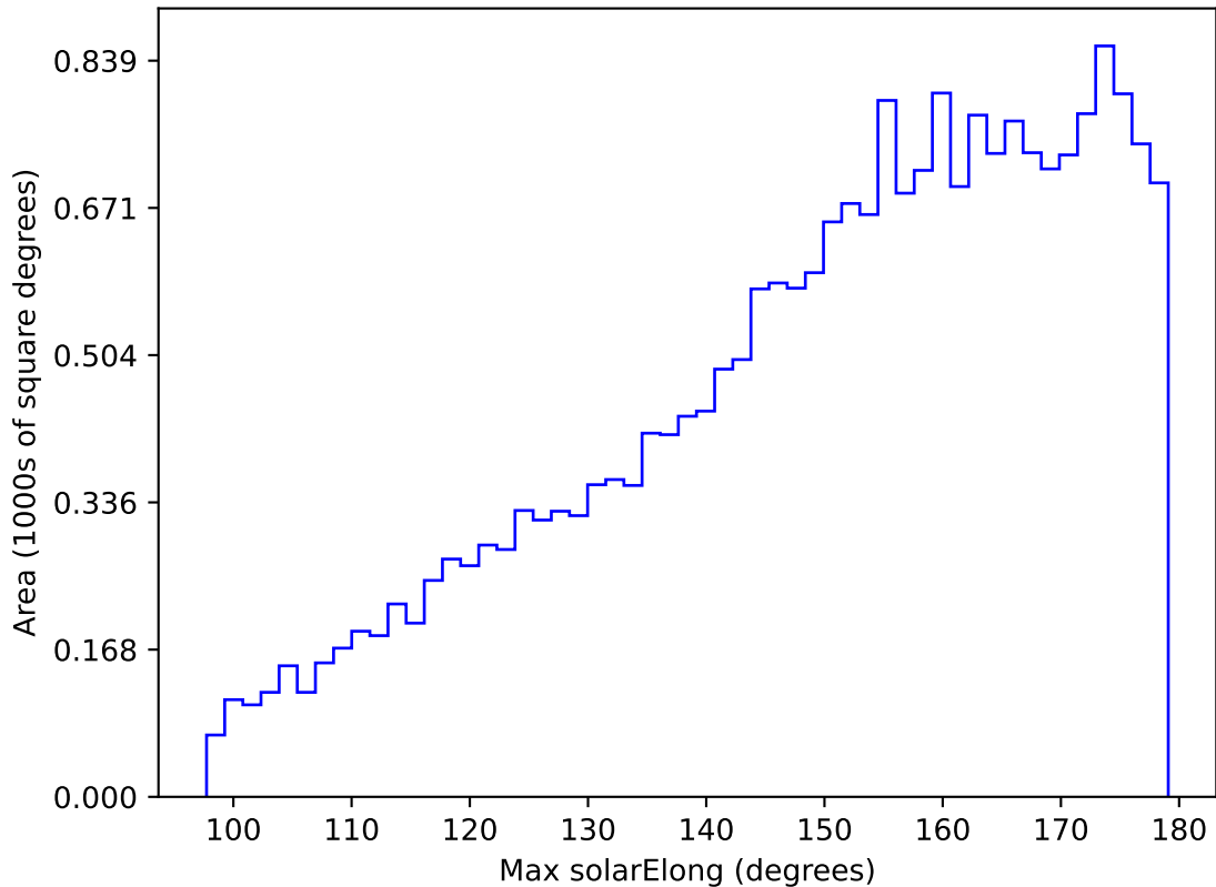
too_elab_r8_d2_ugrizy_v3.4_10yrs All sky u band: Max solarElong
