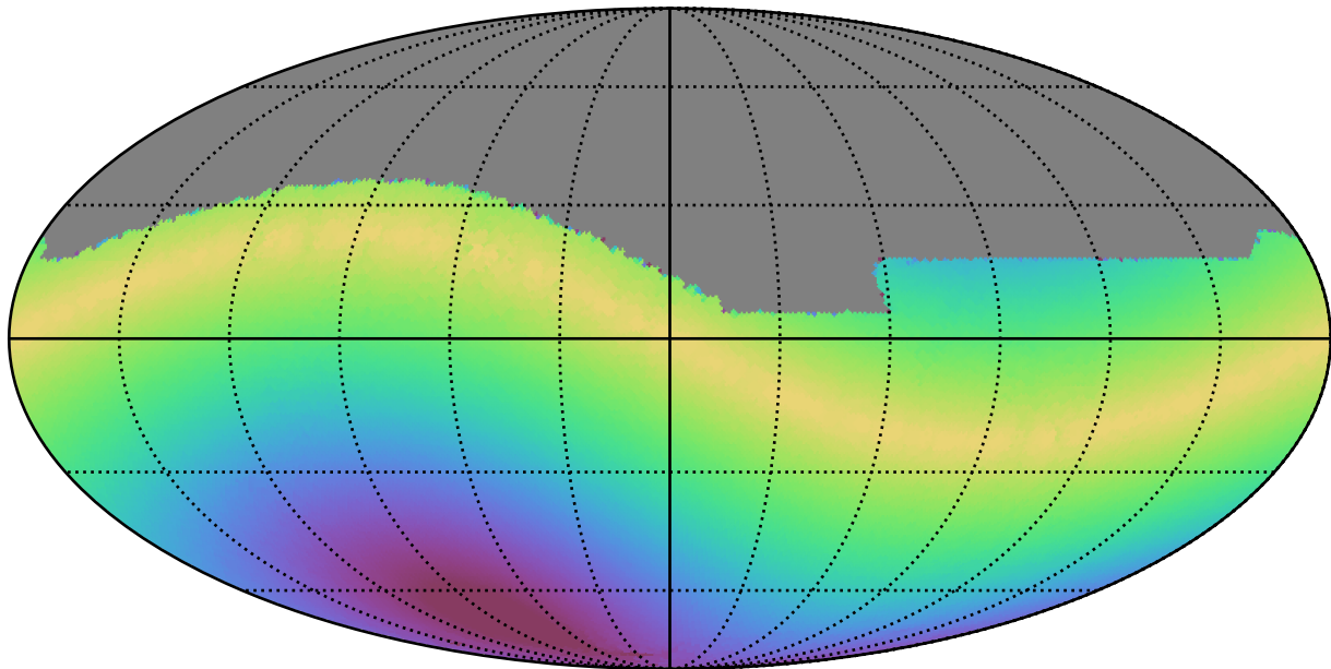
too_elab_r8_d2_ugrizy_v3.4_10yrs All sky r band: Max solarElong
