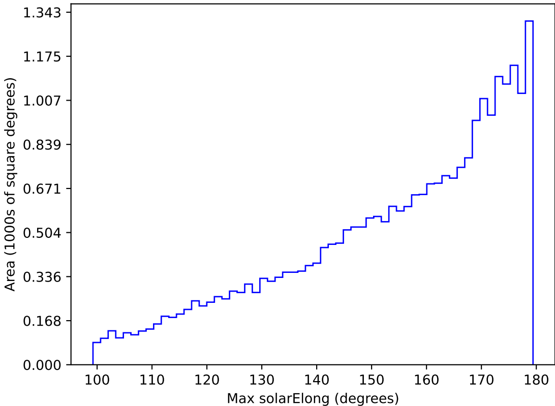
too_elab_r8_d2_ugrizy_v3.4_10yrs All sky i band: Max solarElong
