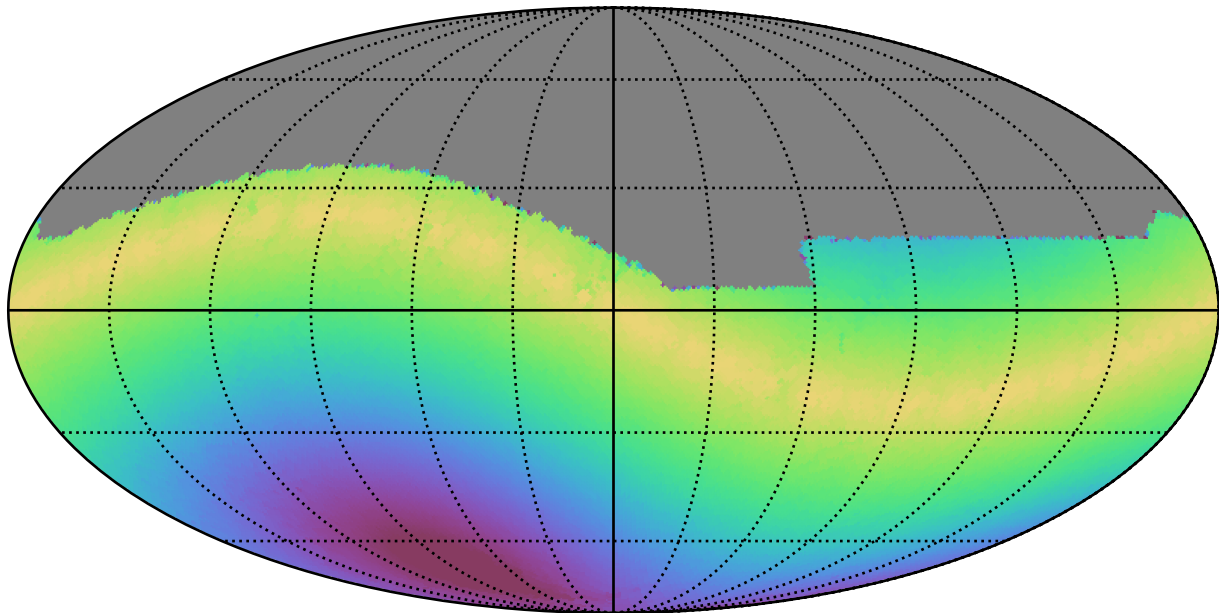
too_elab_r8_d2_ugrizy_v3.4_10yrs All sky g band: Max solarElong
