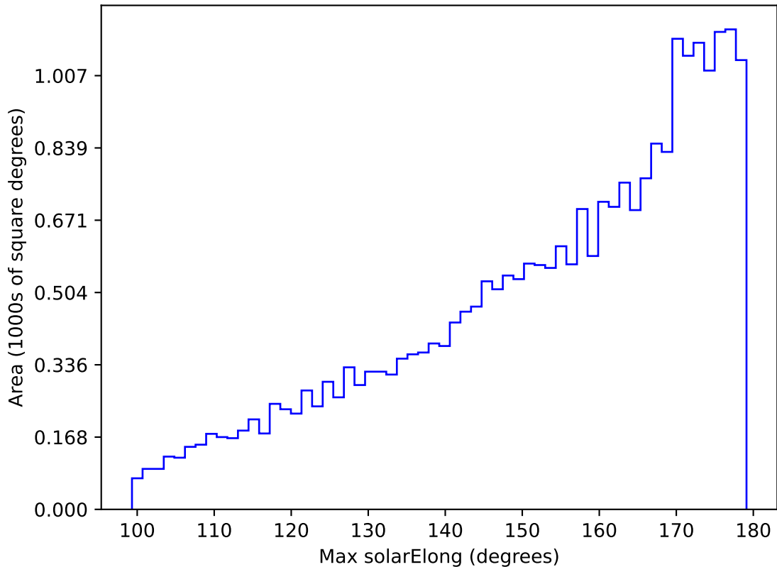
too_elab_r8_d2_ugrizy_v3.4_10yrs All sky g band: Max solarElong
