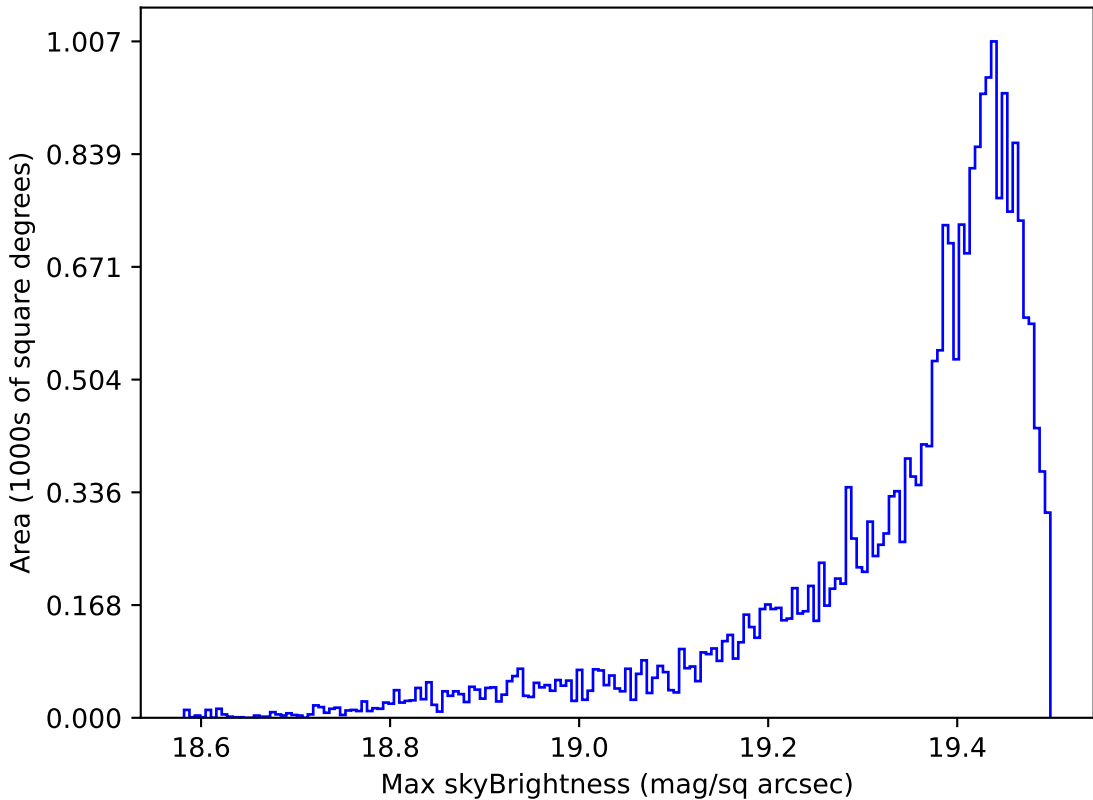
too_elab_r8_d2_ugrizy_v3.4_10yrs Yr 1 z band: Max skyBrightness
